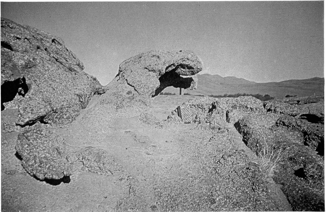
Figure 14. Tafoni in granite at Gobabeb.
