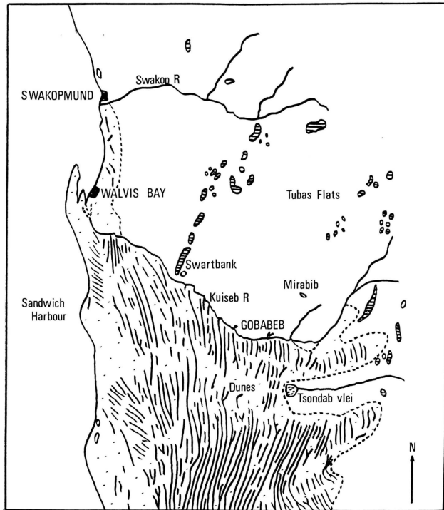
Figure 1. The Central Namib Desert near Gobabeb.
