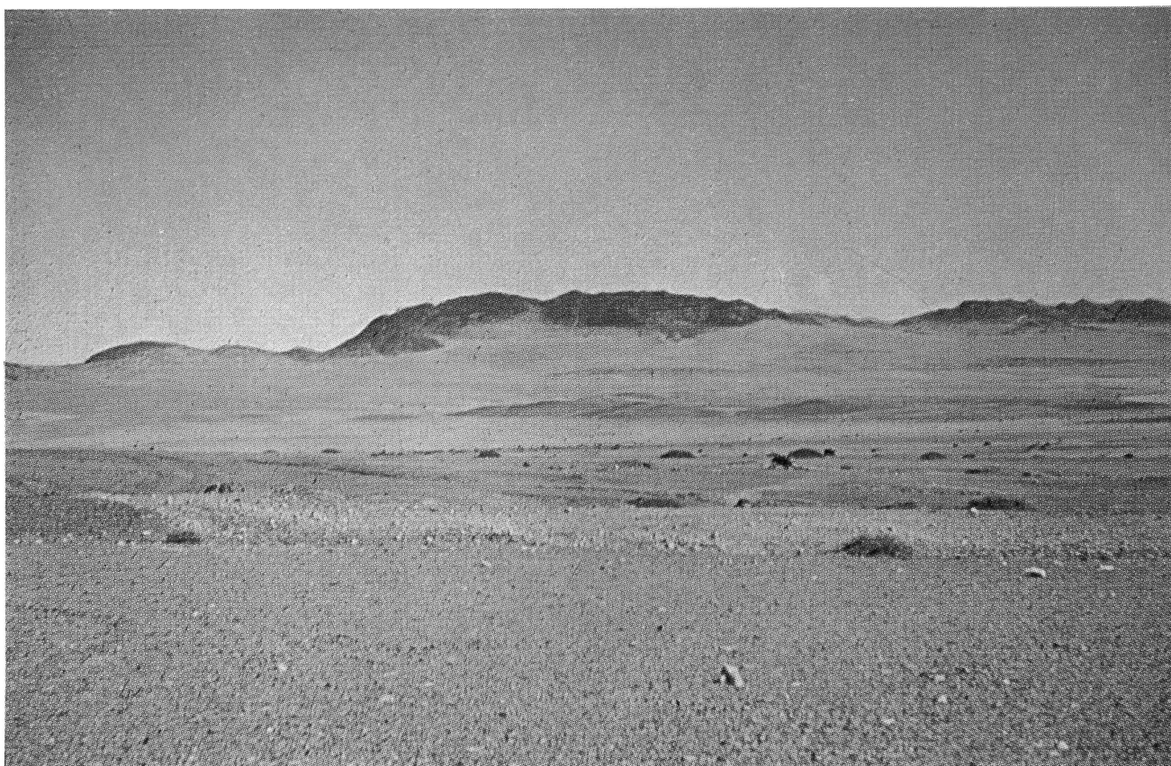
Figure 16. Sand accumulation on the east side of Rössing Mountain.
