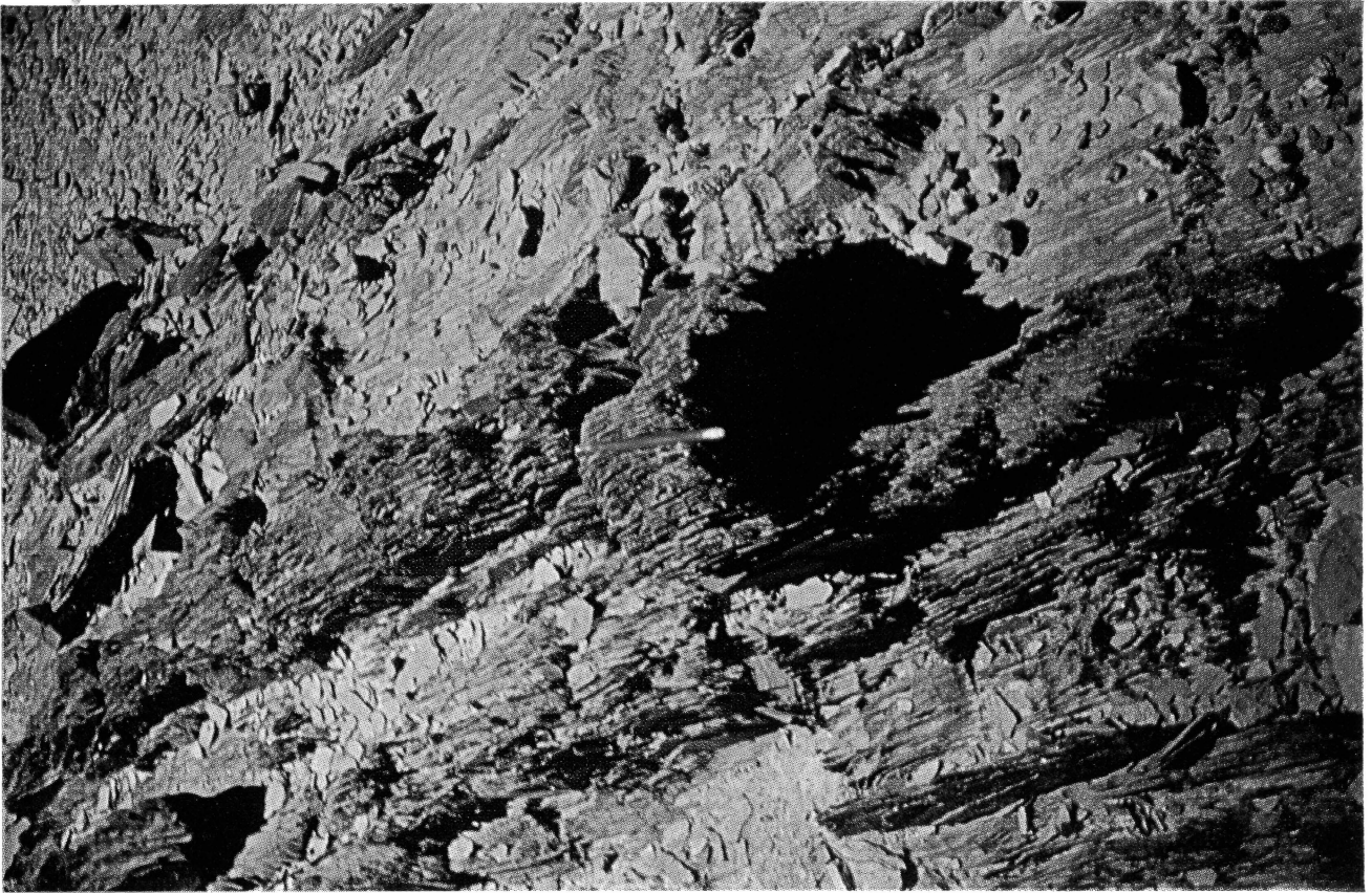
Figure 13. Splitting of schist outcrop near Gobabeb.
